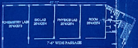
BLOCK - B THIRD FLOOR PLAN BLOCK B COVERED AREA - 1312.90 SQM.
