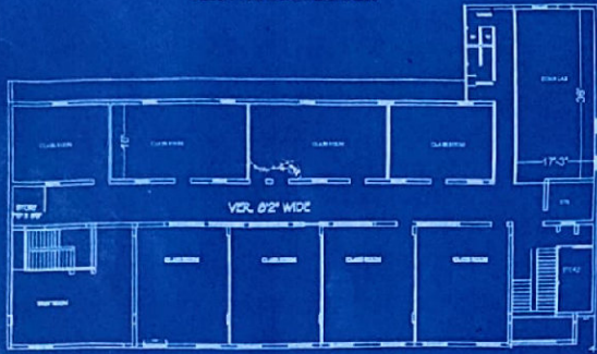
BLOCK - A FIRST FLOOR PLAN
